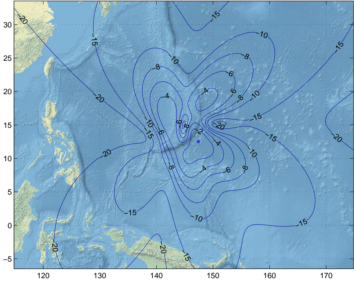
Gain Contours at 505km for GUM. Beam ID=UTX, Polarization=rhcp
