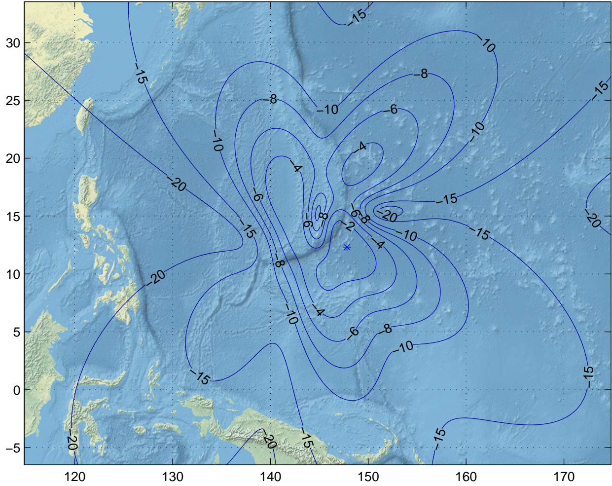
Gain Contours at 575km for GUM. Beam ID=UTX, Polarization=rhcp
