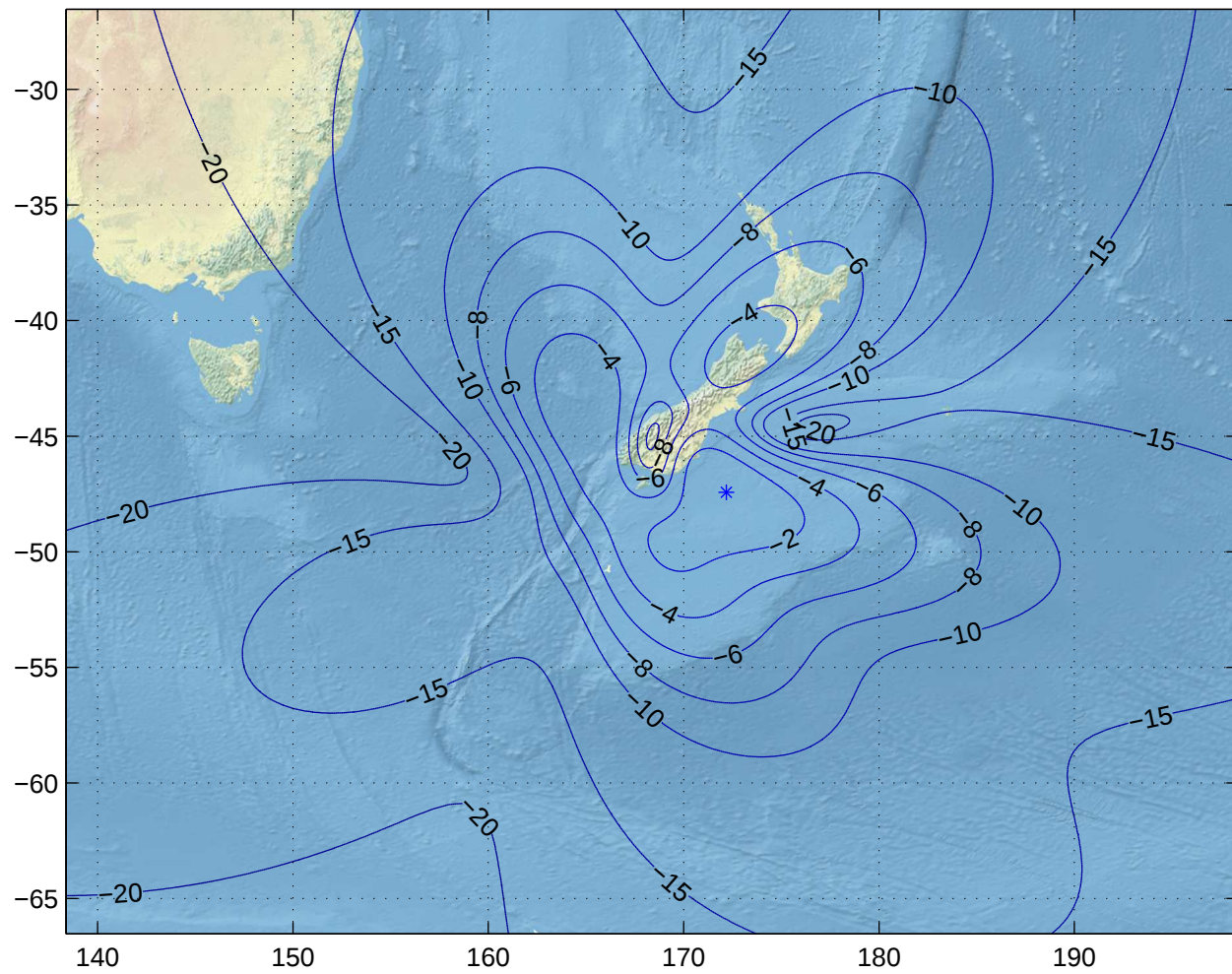
Gain Contours at 505km for IVC. Beam ID=UTX, Polarization=rhcp
