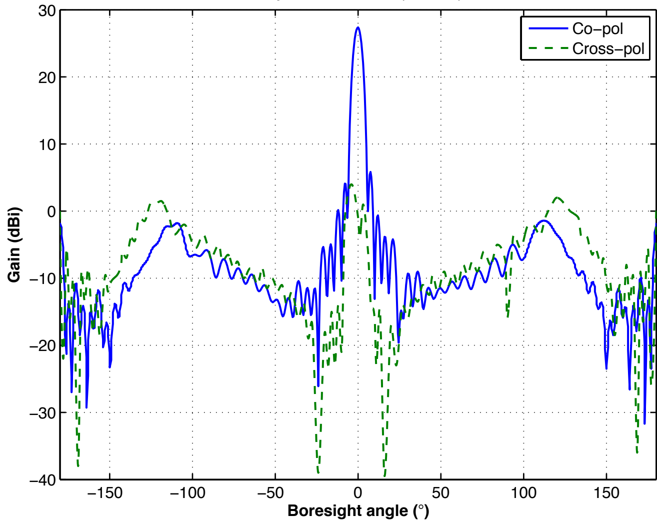
Payload antenna (RHCP)
