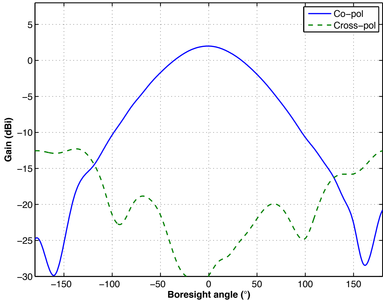
TT&C S-band antenna (RHCP)
