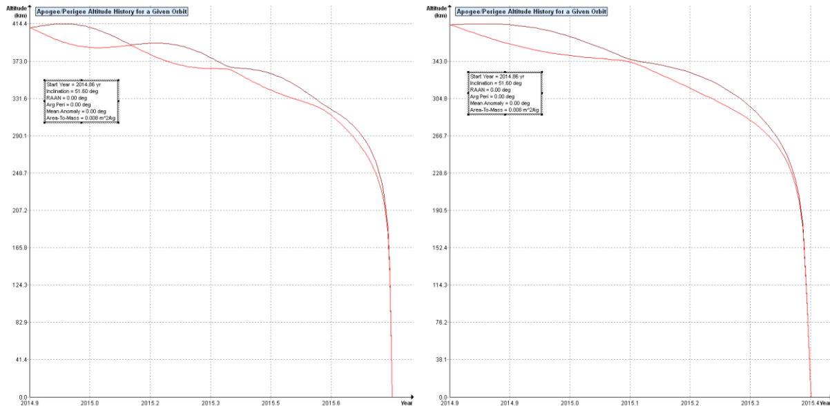
Figure 2: Flock 1d orbit history – High insertion Case (left image) and Low Insertion Case (right image)
