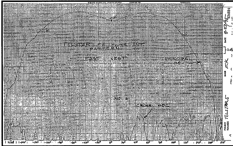
A) Plot Showing Gain Variation In The East-West Direction
