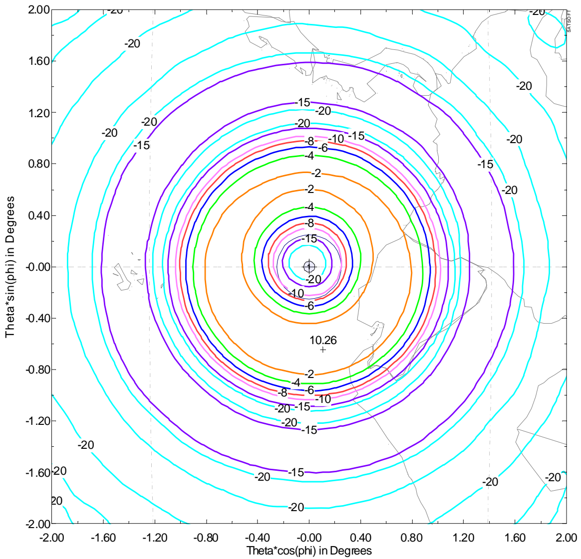
GSO Satellite at 83W Receive Antenna Contours – XPol (Contour Levels: -2, -4, -6, -8, -10, -15, -20 dB)
