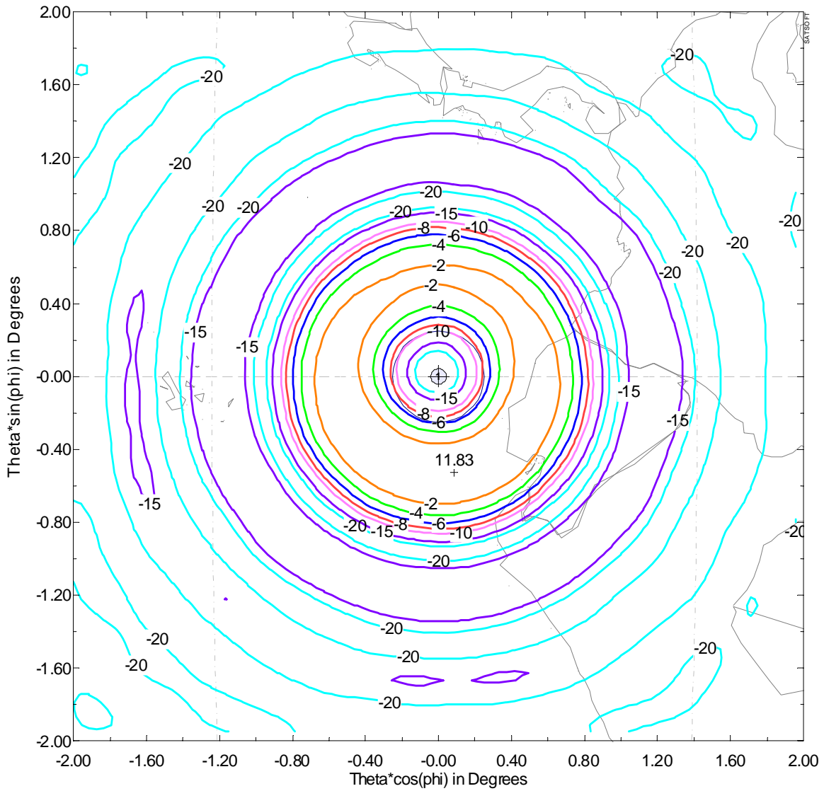
GSO Satellite at 83W Transmit Antenna Contours – XPol (Contour Levels: -2, -4, -6, -8, -10, -15, -20 dB)
