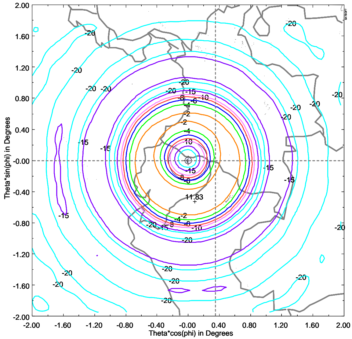
GSO Satellite at 77W Transmit Antenna Contours – XPol (Contour Levels: -2, -4, -6, -8, -10, -15, -20 dB)
