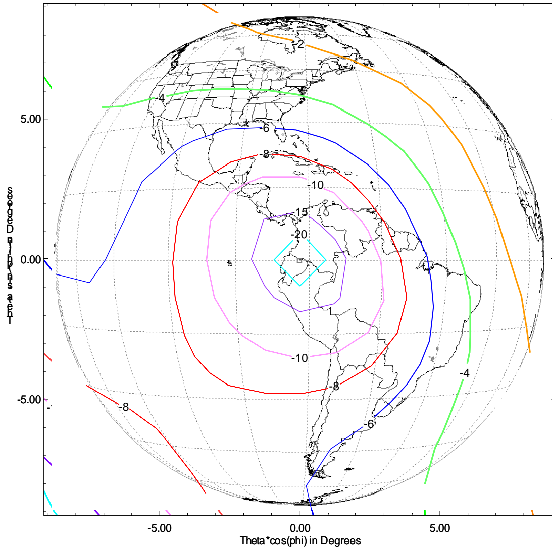
Figure C6: Beacon Contours Transmit and Receive (Xpol)
