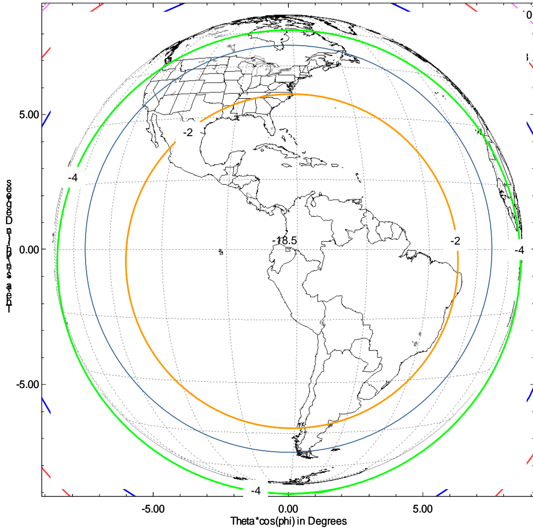
Figure C5: Beacon Contours Transmit and Receive (Copol)
