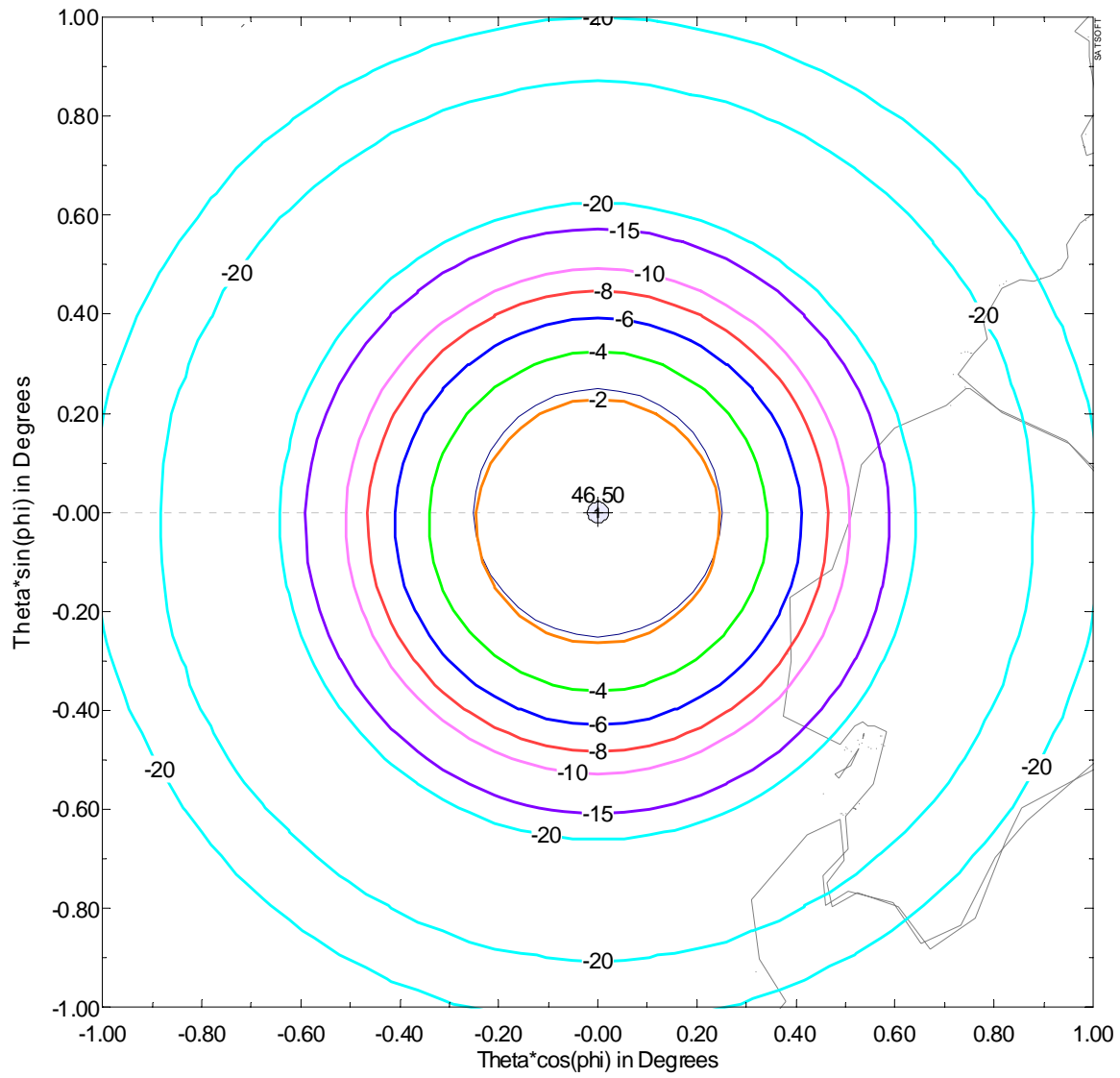
GSO Satellite Receive Antenna Contours – CoPol (Contour levels: -2, -4, -6, -8, -10, -15, - 20 dB)
