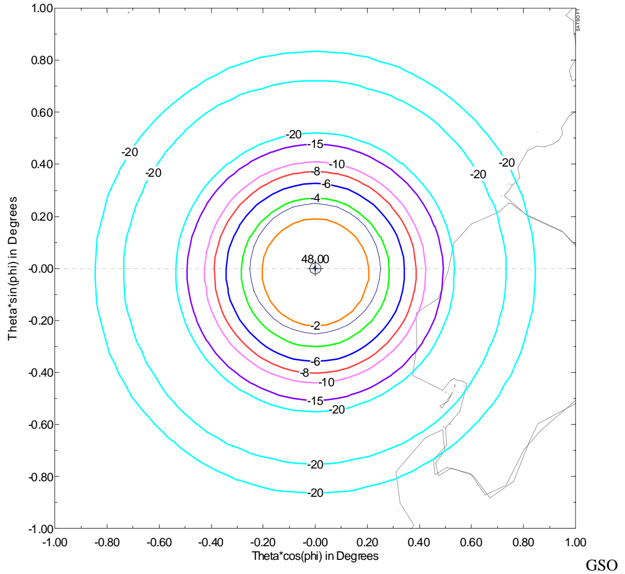
GSO Satellite Transmit Antenna Contours – CoPol (Contour levels: -2, -4, -6, -8, -10, -15, -20 dB)
