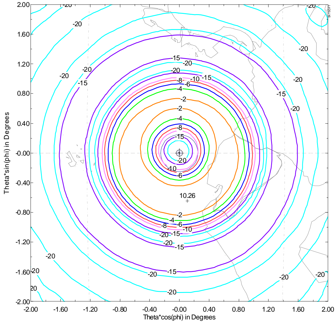
GSO Satellite Receive Antenna Contours – XPol (Contour levels: -2, -4, -6, -8, -10, -15, -20 dB)
