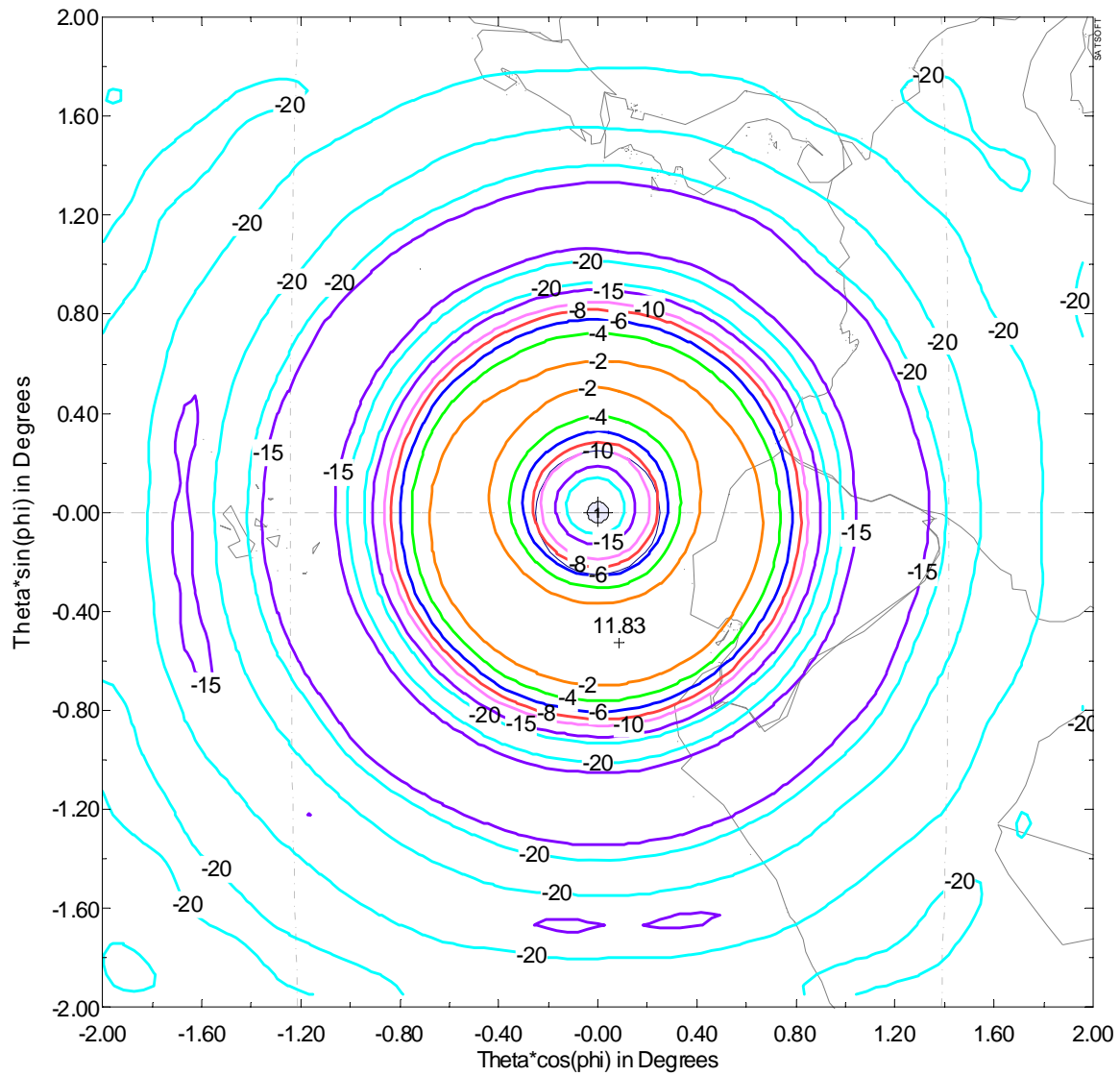
GSO Satellite Transmit Antenna Contours – XPol (Contour levels: -2, -4, -6, -8, -10, -15, -20 dB)
