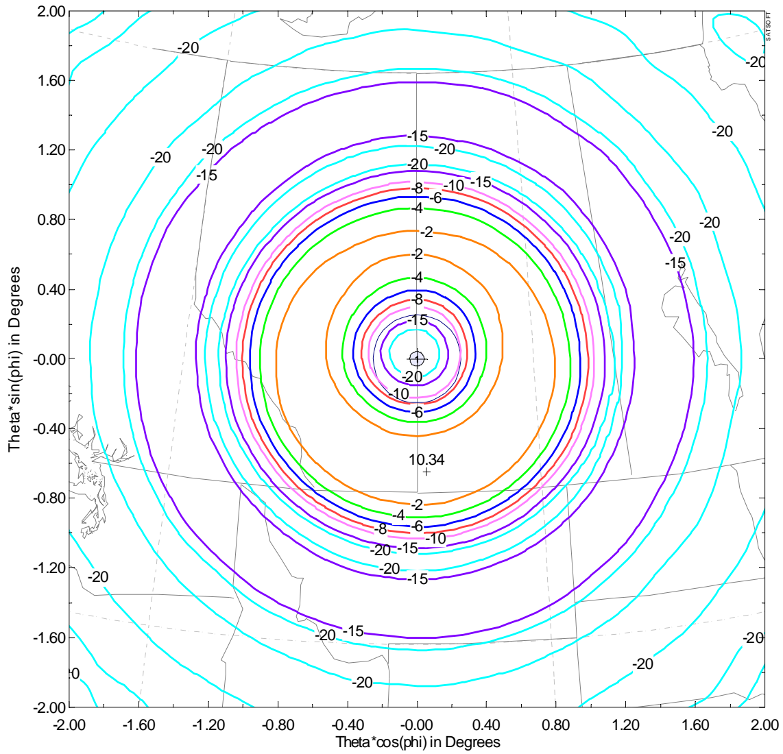
HEO Satellite Receive Antenna Contours – XPol (52.5 N, 109.98 W, 29015 km) (Contour levels: -2, -4, -6, -8, -10, -15, -20 dB)
