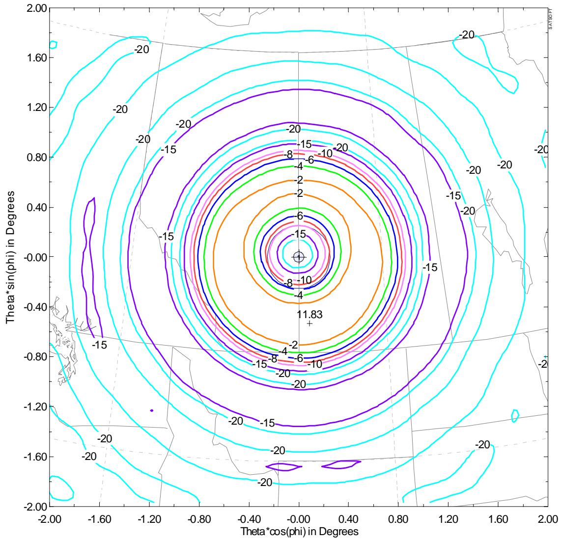
HEO Satellite Transmit Antenna Contours – XPol (52.5 N, 109.98 W, 29015 km) (Contour levels: -2, -4, -6, -8, -10, -15, -20 dB)
