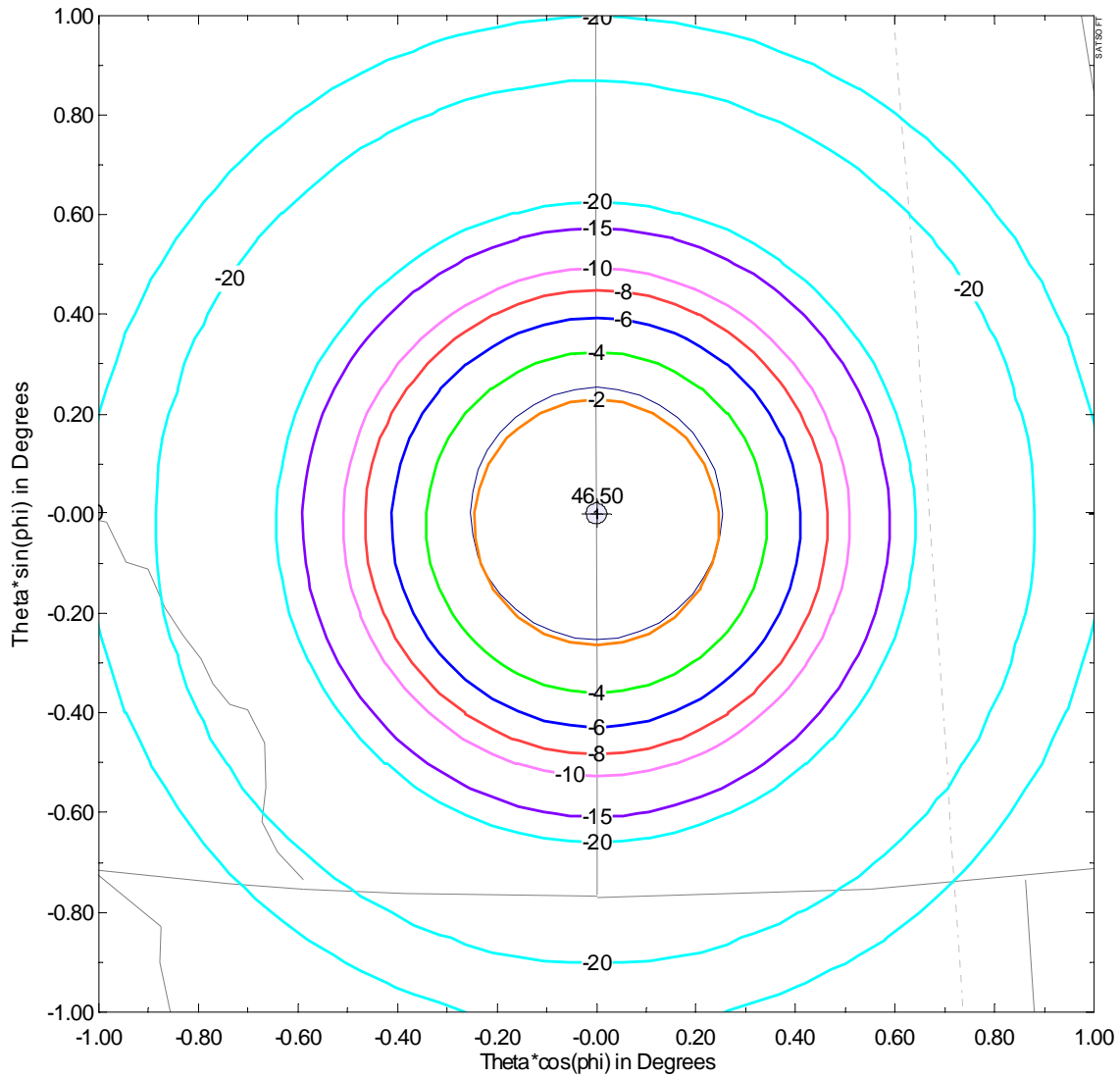
HEO Satellite Receive Antenna Contours – CoPol (52.5 N, 109.98 W, 29015 km) (Contour levels: -2, -4, -6, -8, -10, -15, -20 dB)
