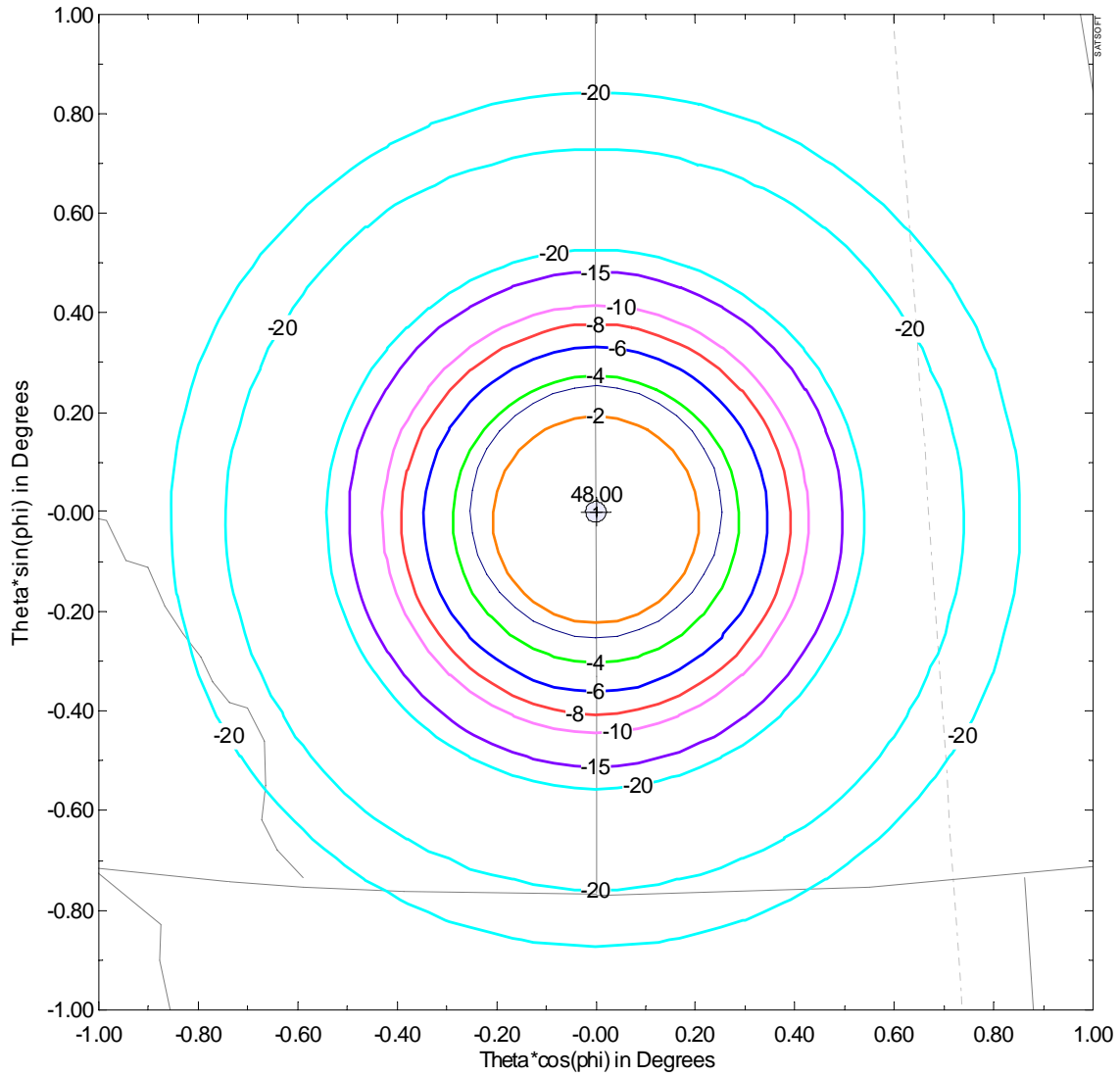
HEO Satellite Transmit Antenna Contours – CoPol (52.5 N, 109.98 W, 29015 km) (Contour levels: -2, -4, -6, -8, -10, -15, - 20 dB)
