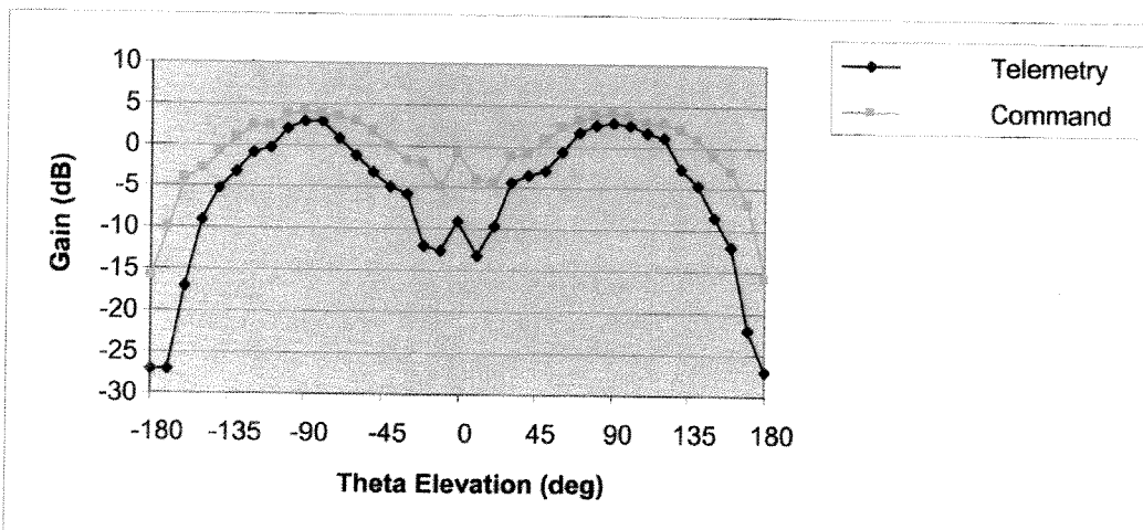
Gain vs. Elevation Angle (Azimuth Angle of 0°)
