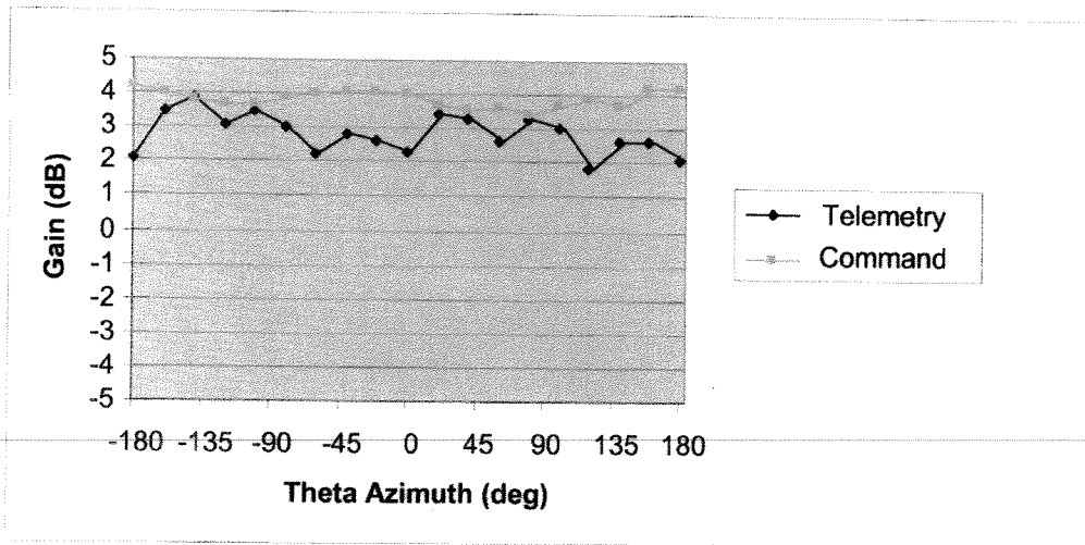
Gain vs. Azimuth (Elevation Angle of 90°)
