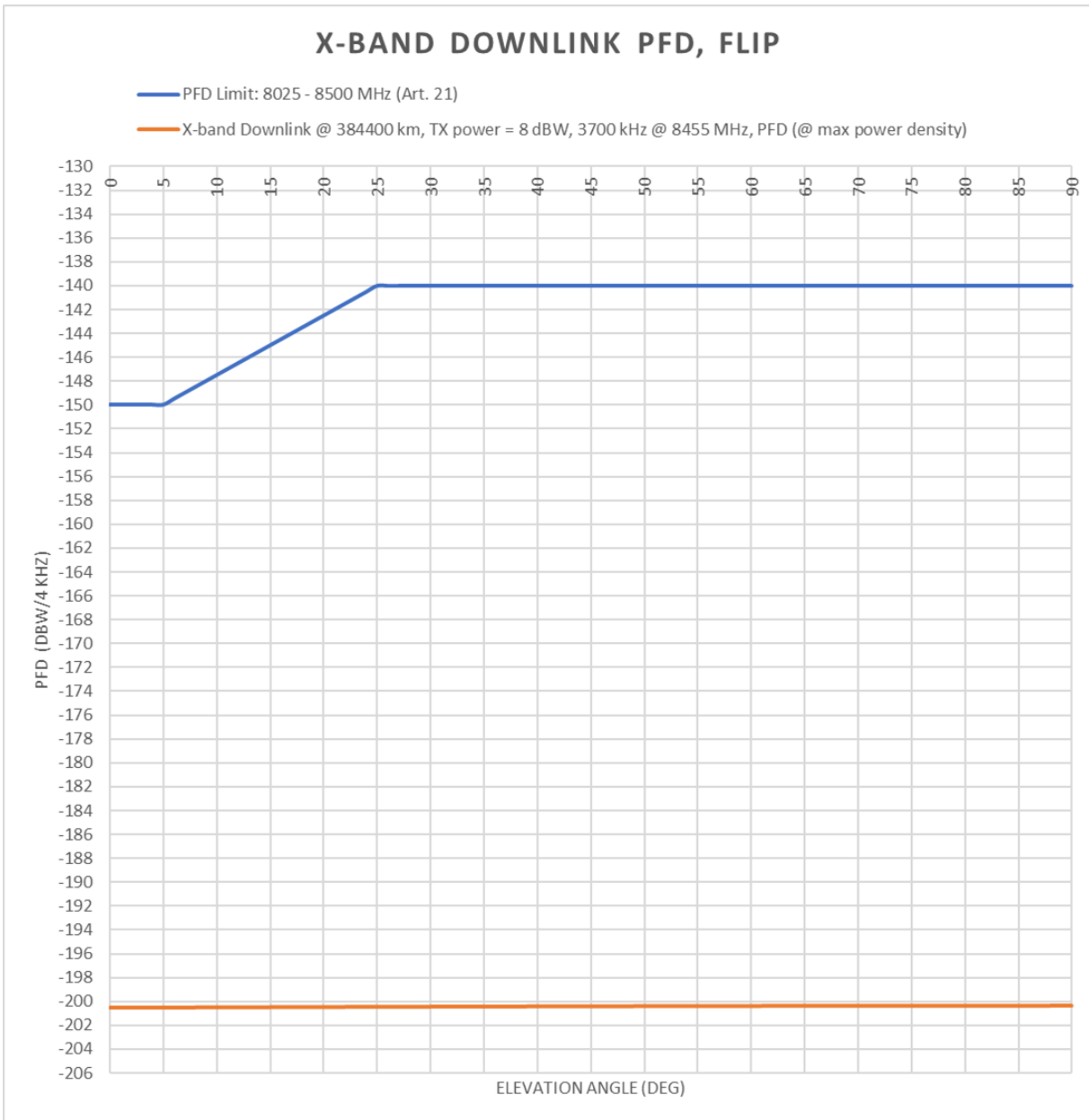
Figure 2: X-band downlink power flux density (PFD) from the FLIP rover assuming 12 dBW peak EIRP. Only free-space path loss is included. Value is shown for transmission from the lunar south pole only.
