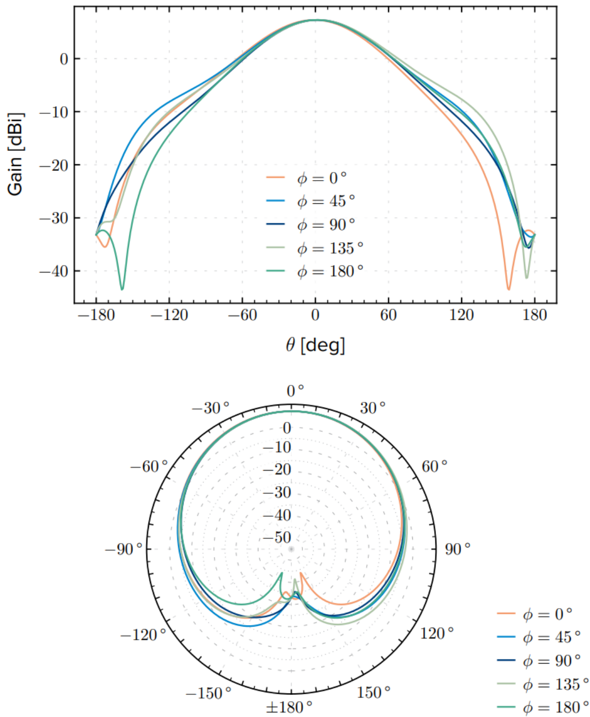
Figure 5: Simulated Radiation Pattern of the antenna at 2.07 GHz
