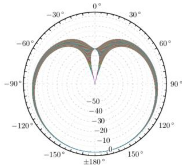
Figure 1: LHCP Radiation Pattern
