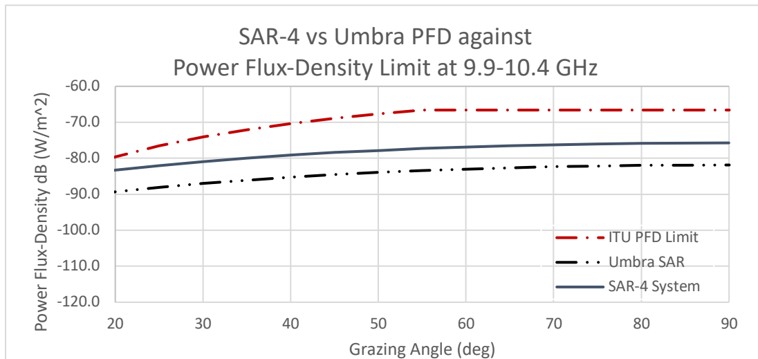
Figure 1. Comparison of Mean PFD Values and PFD Limit
