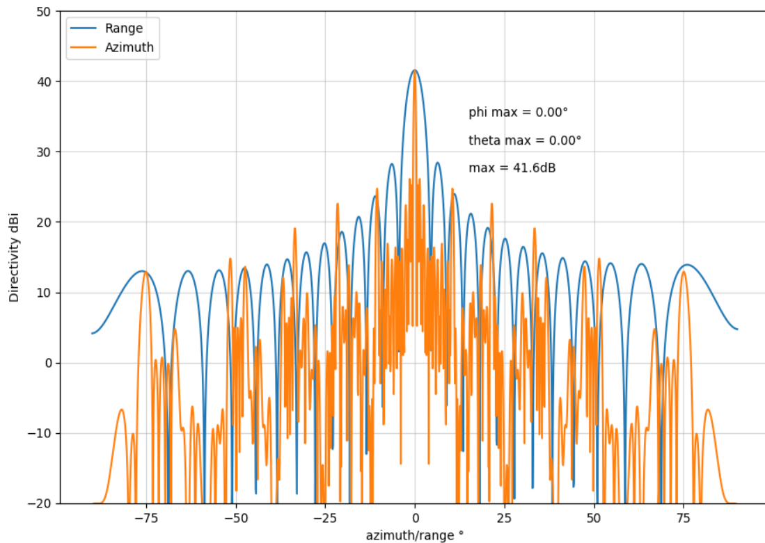
Figure 1: Typical SAR Transmit/Receive Beam Pattern
