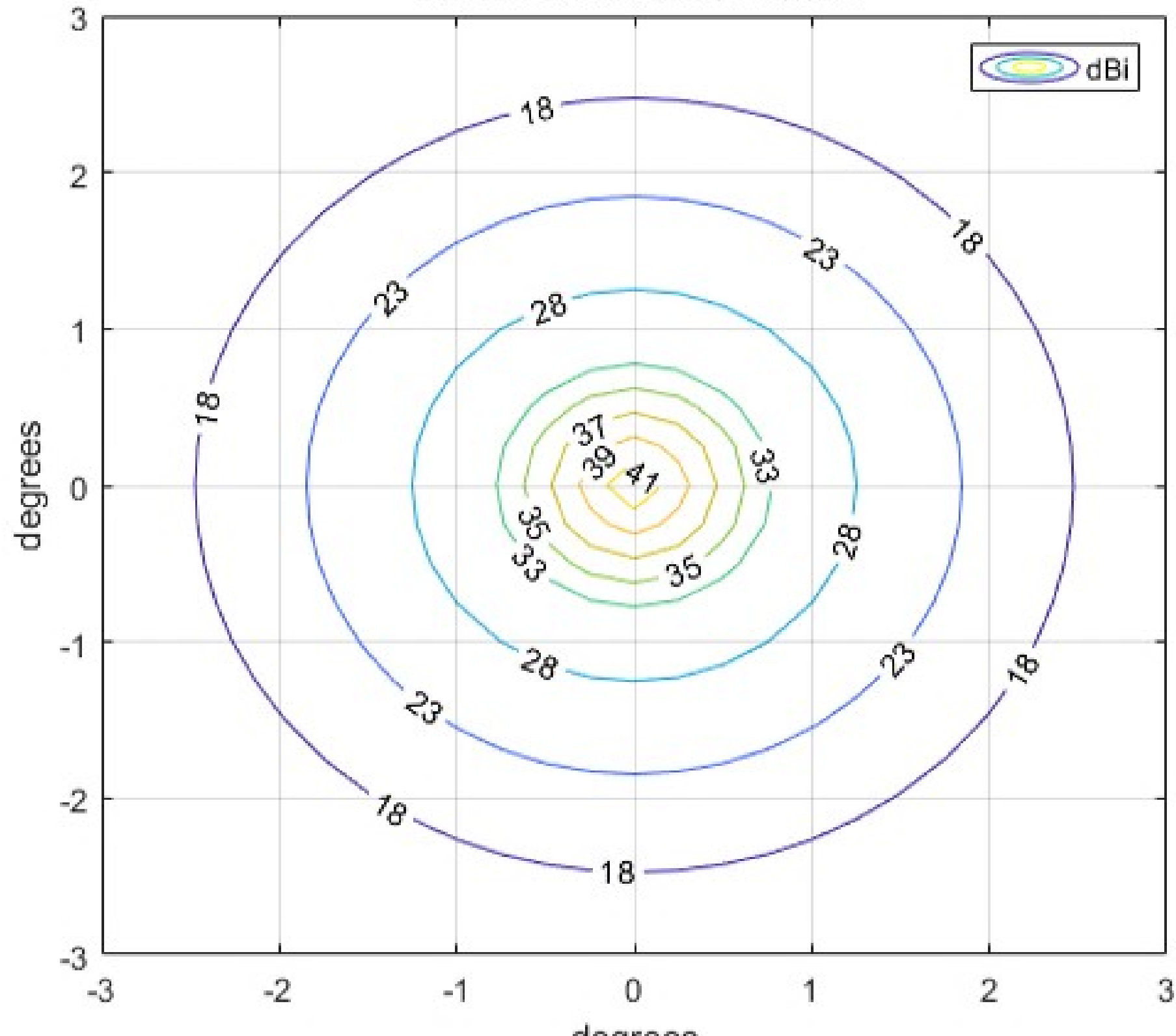
Ka-Band Transmit Pattern
