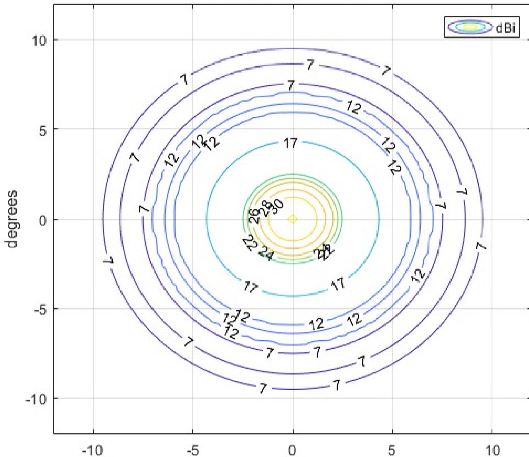
X-Band Receive Pattern
