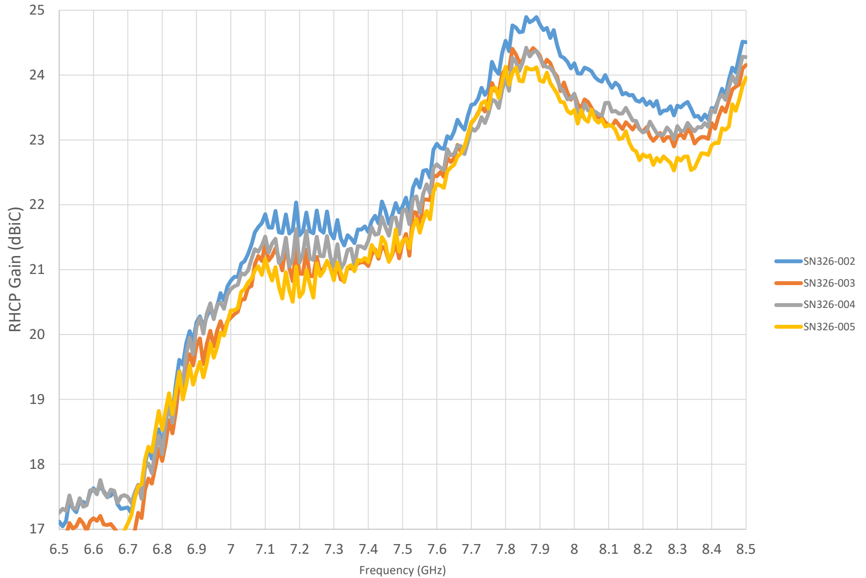
Broadside RHCP Gain (dBiC) vs Frequency
