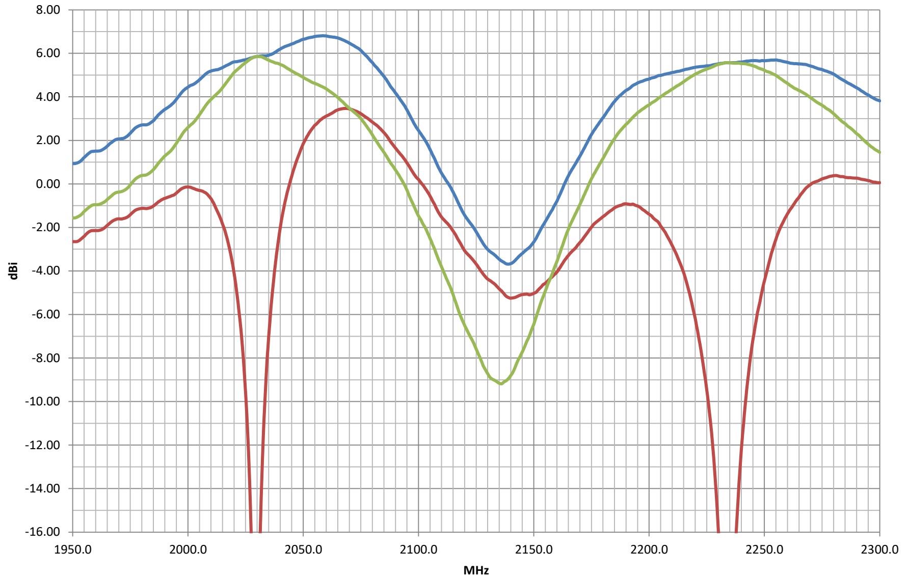
Broadside +Z Axis Gains in dBi
