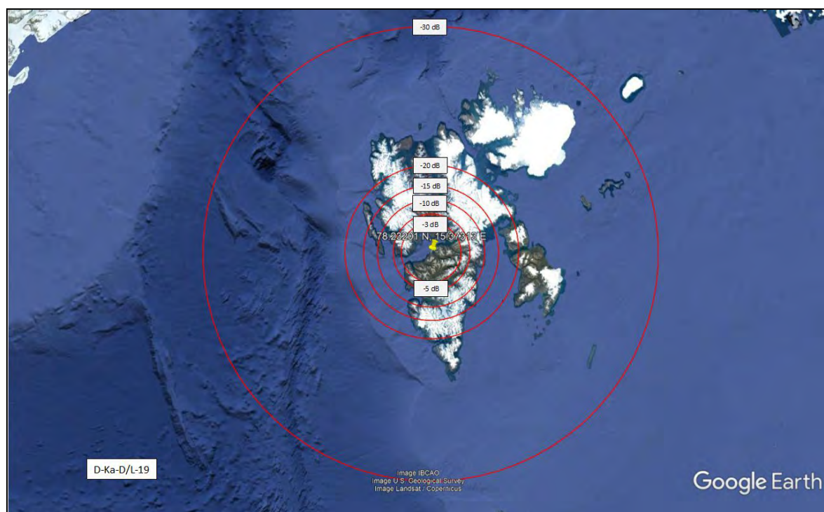
Figure A.5-2 KaG and KaH transmit antenna gain contours - Svalbard
