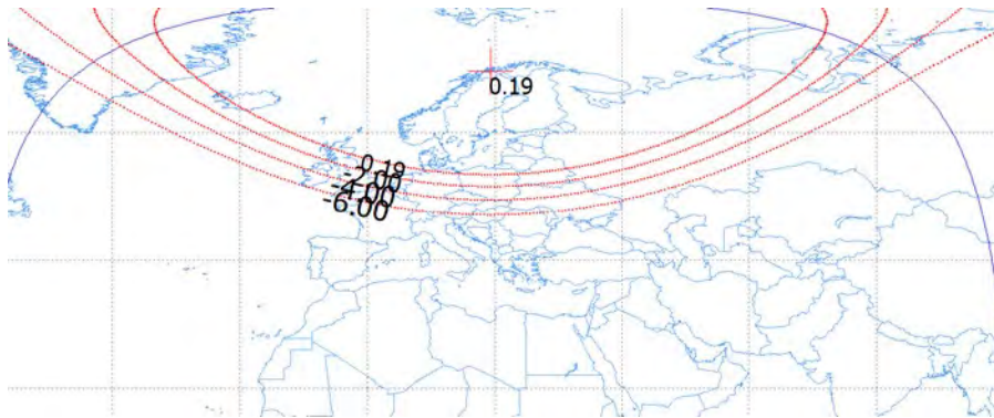
Figure A.5-10 UTLM receive antenna gain contours – Tromsø
