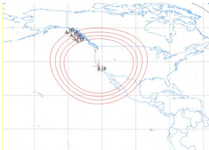
Figure A.5-9 UTLM receive antenna gain contours – Santa Clara
