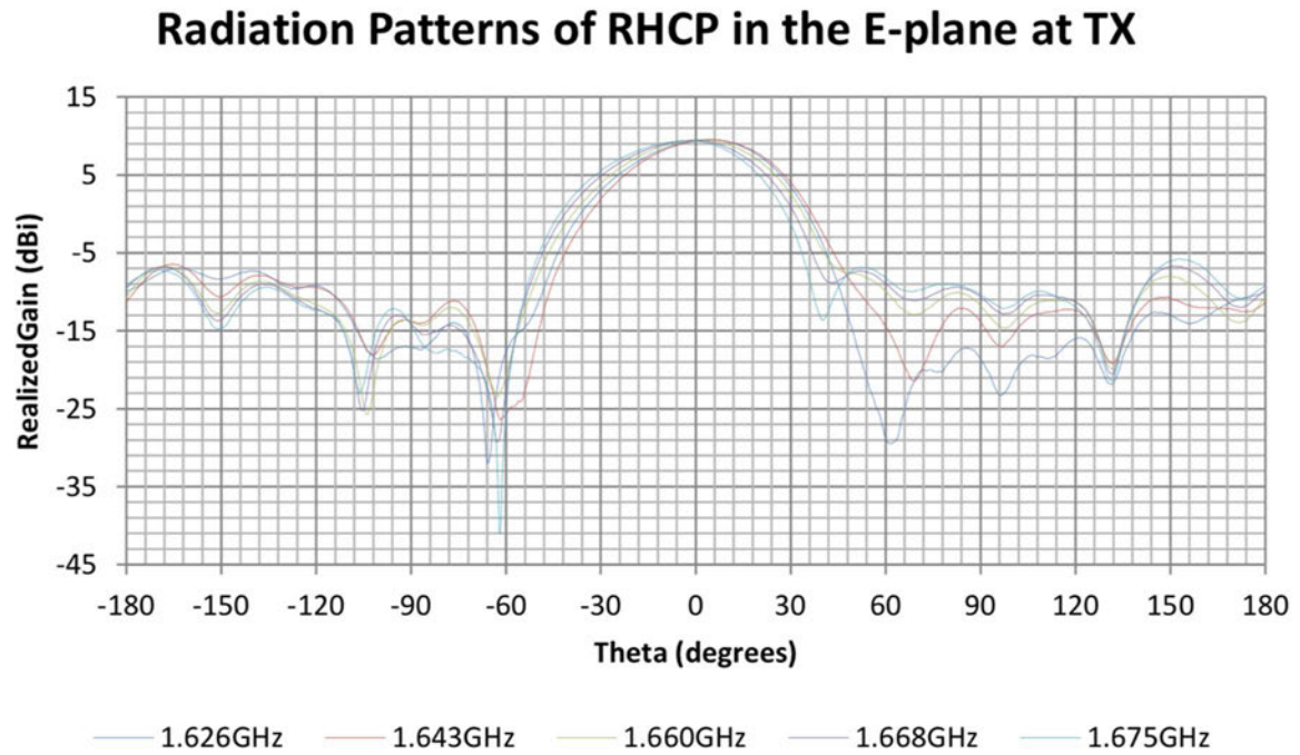
Figure V.F-1. Capella Space-to-Space Downlink E-Plane Gain Pattern
