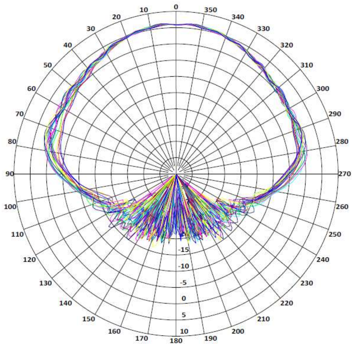
Gain (dBic) vs. Angle
