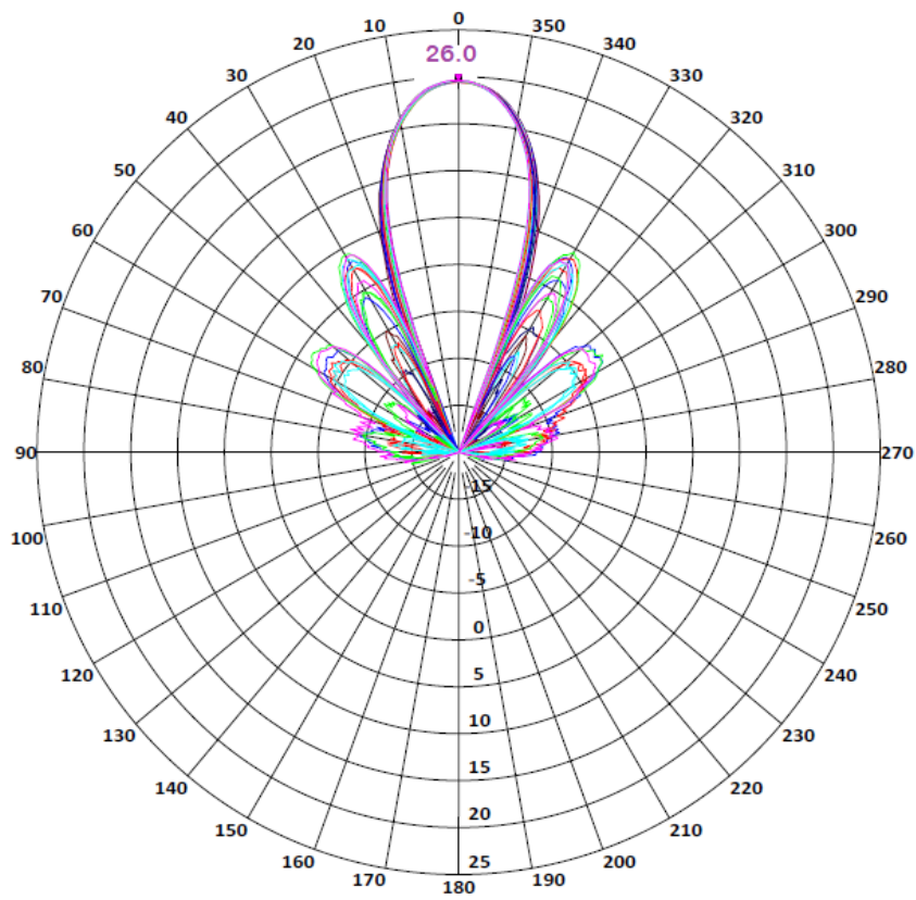
Gain (dBic) vs. Angle
