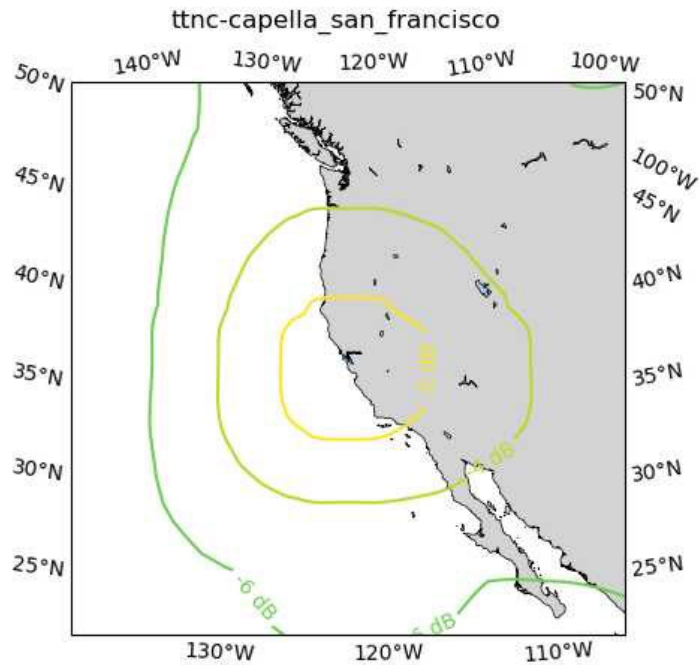
Figure V.B-2. Capella X-Band TT&C Downlink Ground-Projected Gain Contours for 575 km Altitude
