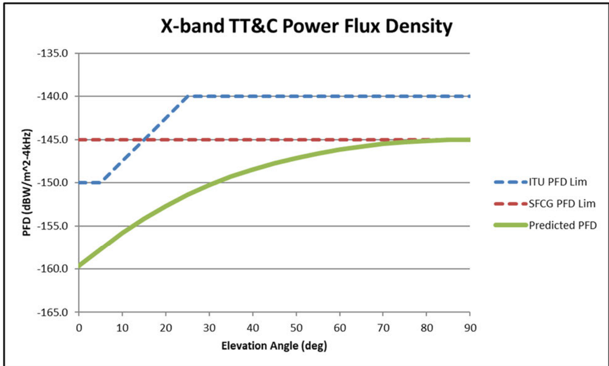
Figure VII.A-2. Capella X-Band TT&C Downlink PFD at Earth Surface
