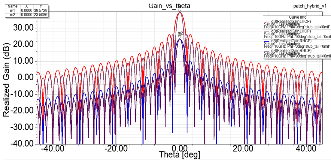
Figure 2: SAR beampattern (short side)
