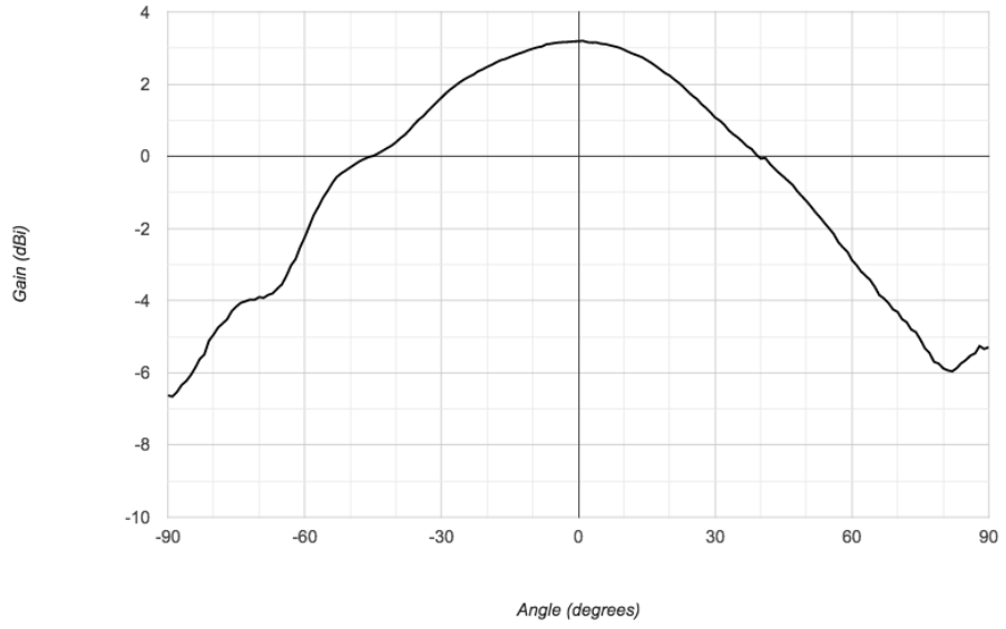
S-Band Patch Horizontal Cut, Vertical Polarization
