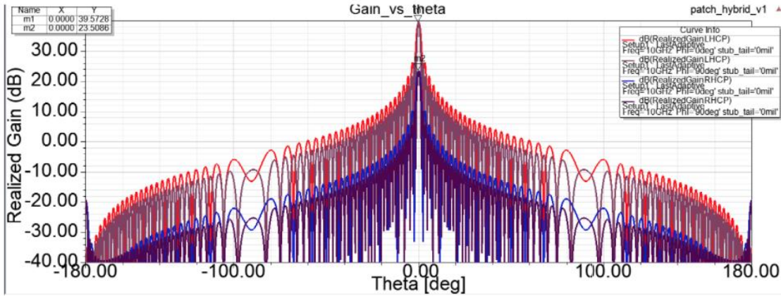
Figure 1: SAR Beampattern (long side)
