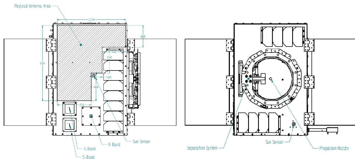
Figure 3: HE360 External Layout -Y and -X Views
