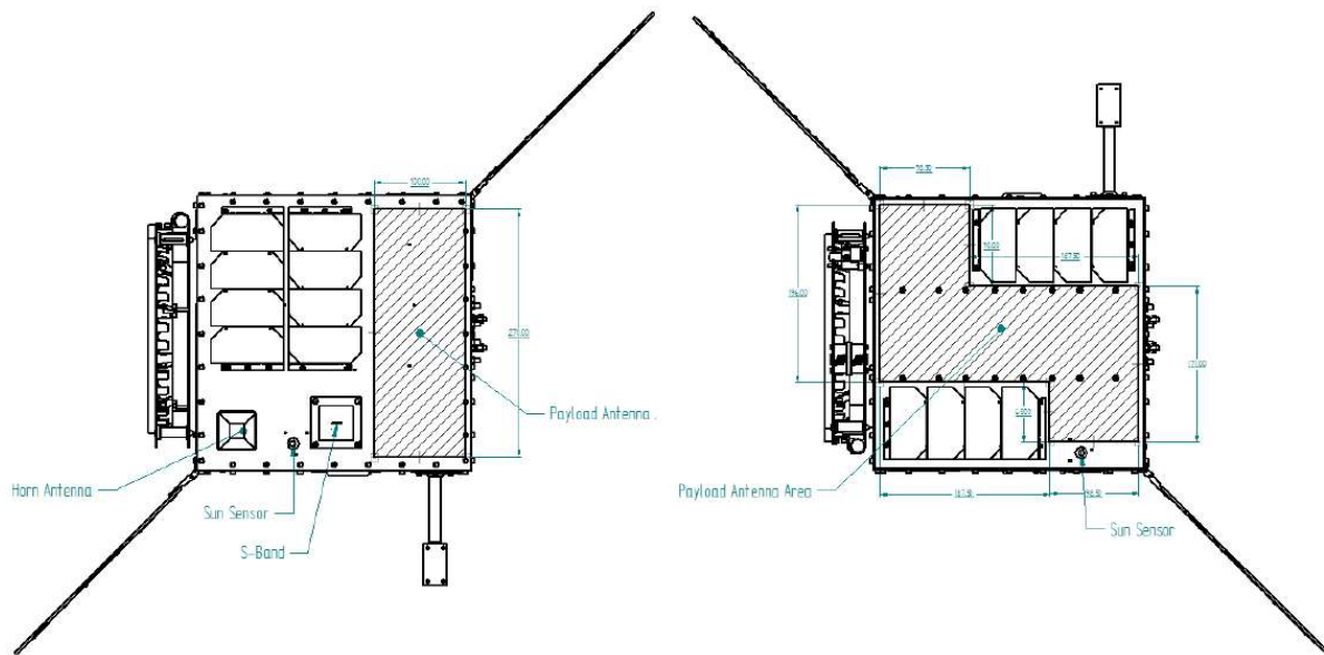
Figure 4: HE360 External Layout +Z and -Z Views
