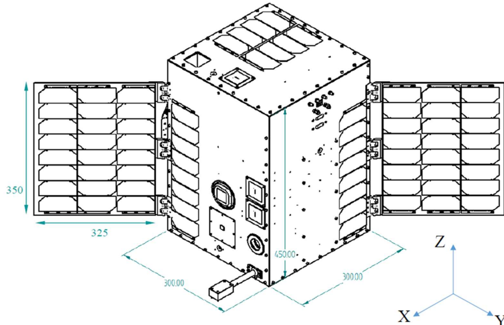
Figure 1: HE360 External Layout
