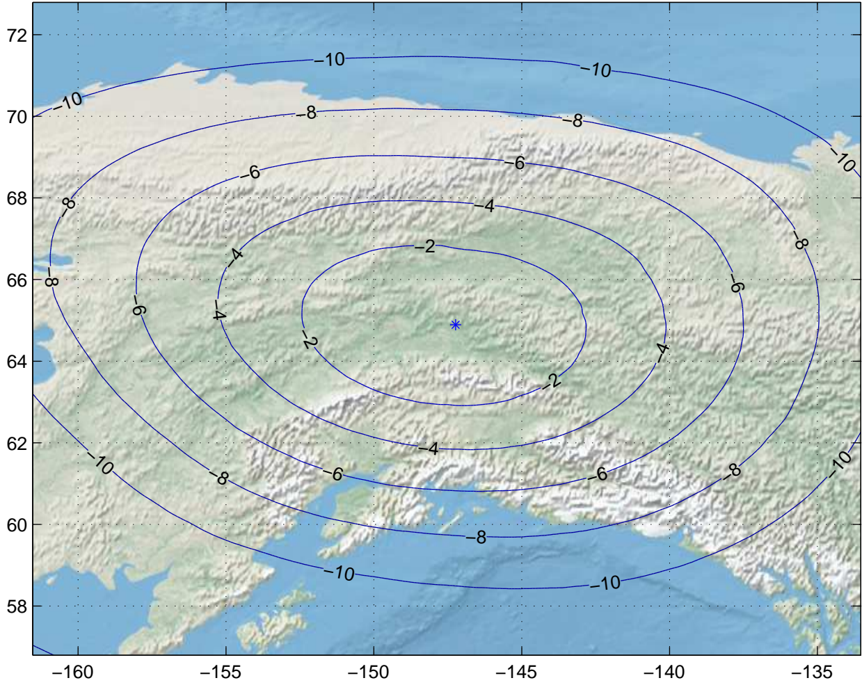
Gain Contours at 460km for FAI. Beam ID=SRC, Polarization=rhcp
