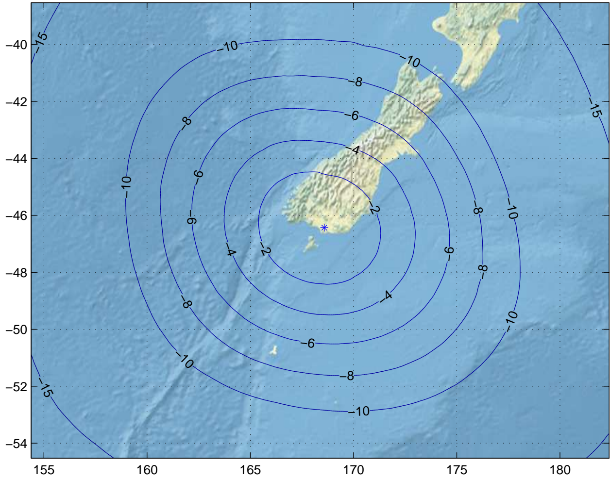
Gain Contours at 460km for IVC. Beam ID=SRC, Polarization=rhcp
