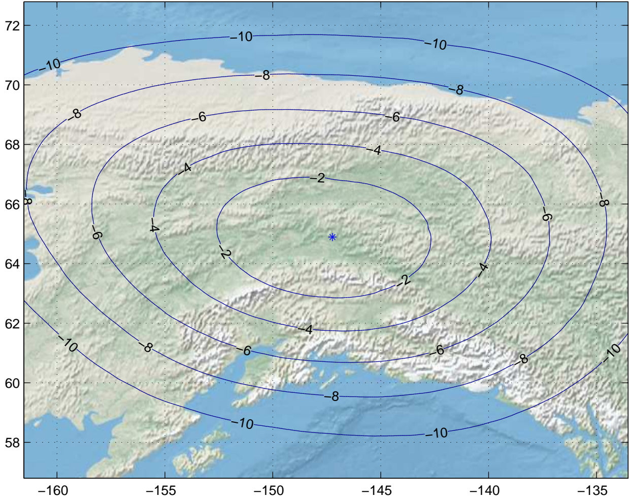
Gain Contours at 475km for FAI. Beam ID=SRC, Polarization=rhcp
