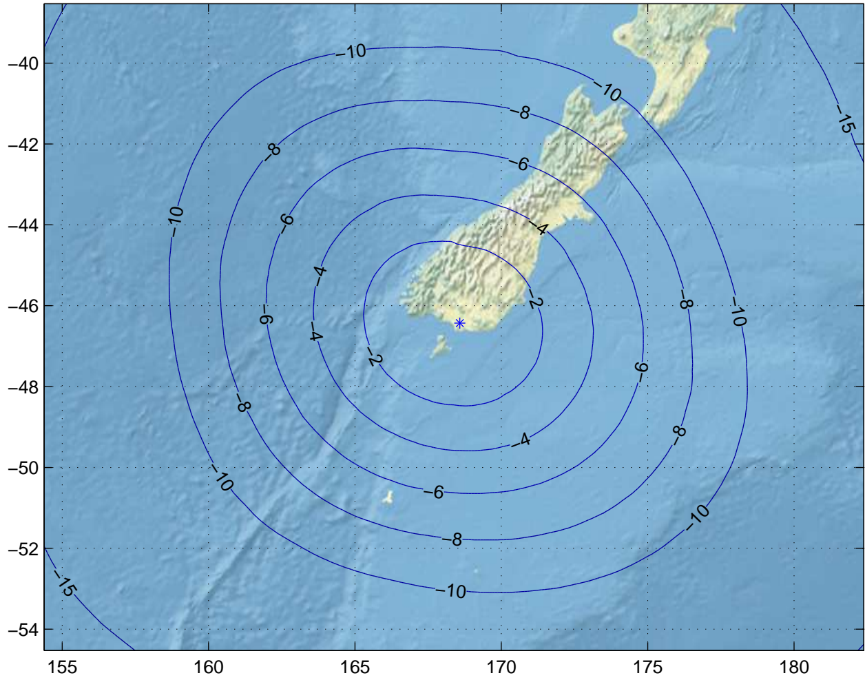
Gain Contours at 475km for IVC. Beam ID=SRC, Polarization=rhcp
