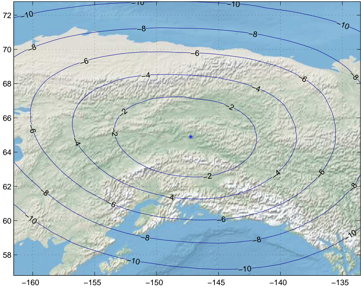
Gain Contours at 550km for FAI. Beam ID=SRC, Polarization=rhcp
