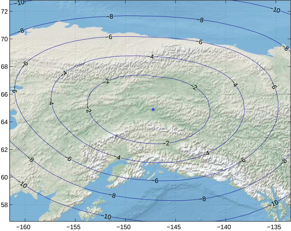
Gain Contours at 585km for FAI. Beam ID=SRC, Polarization=rhcp
