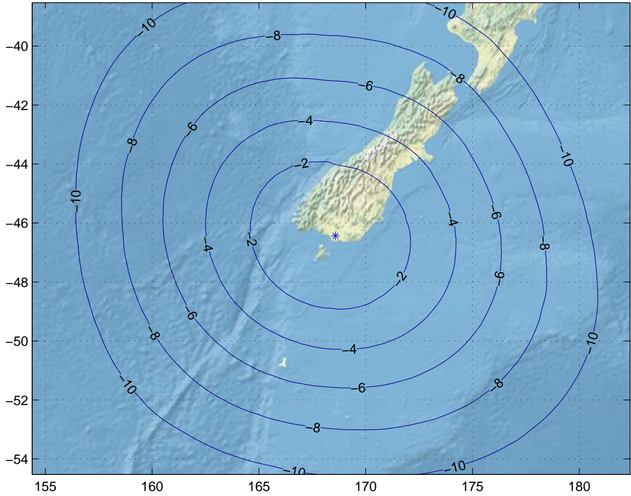
Gain Contours at 585km for IVC. Beam ID=SRC, Polarization=rhcp
