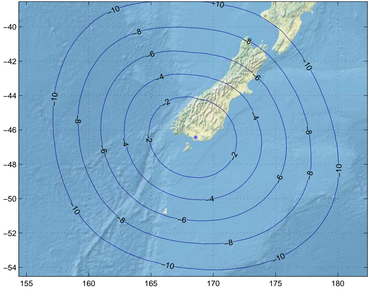
Gain Contours at 550km for IVC. Beam ID=SRC, Polarization=rhcp
