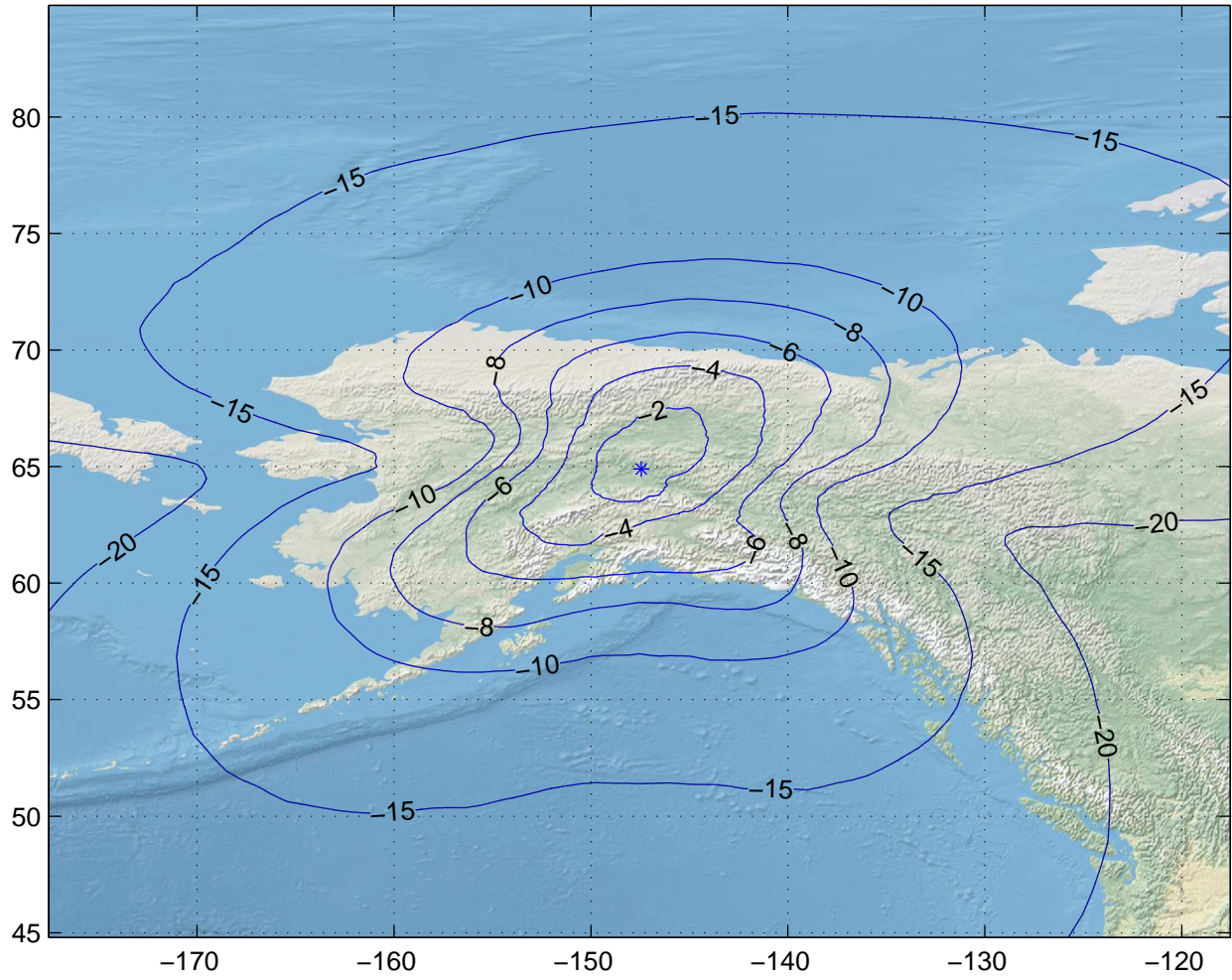
Gain Contours at 460km for FAI. Beam ID=SRX, Polarization=lhcp
