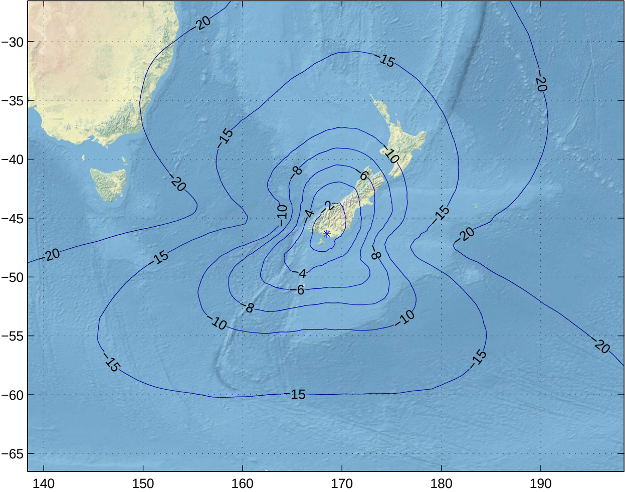
Gain Contours at 460km for IVC. Beam ID=SRX, Polarization=lhcp
