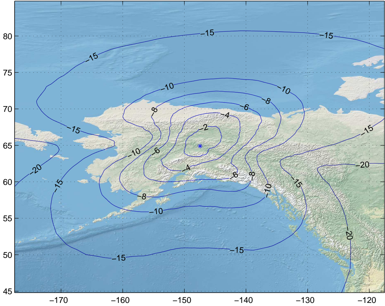
Gain Contours at 475km for FAI. Beam ID=SRX, Polarization=lhcp
