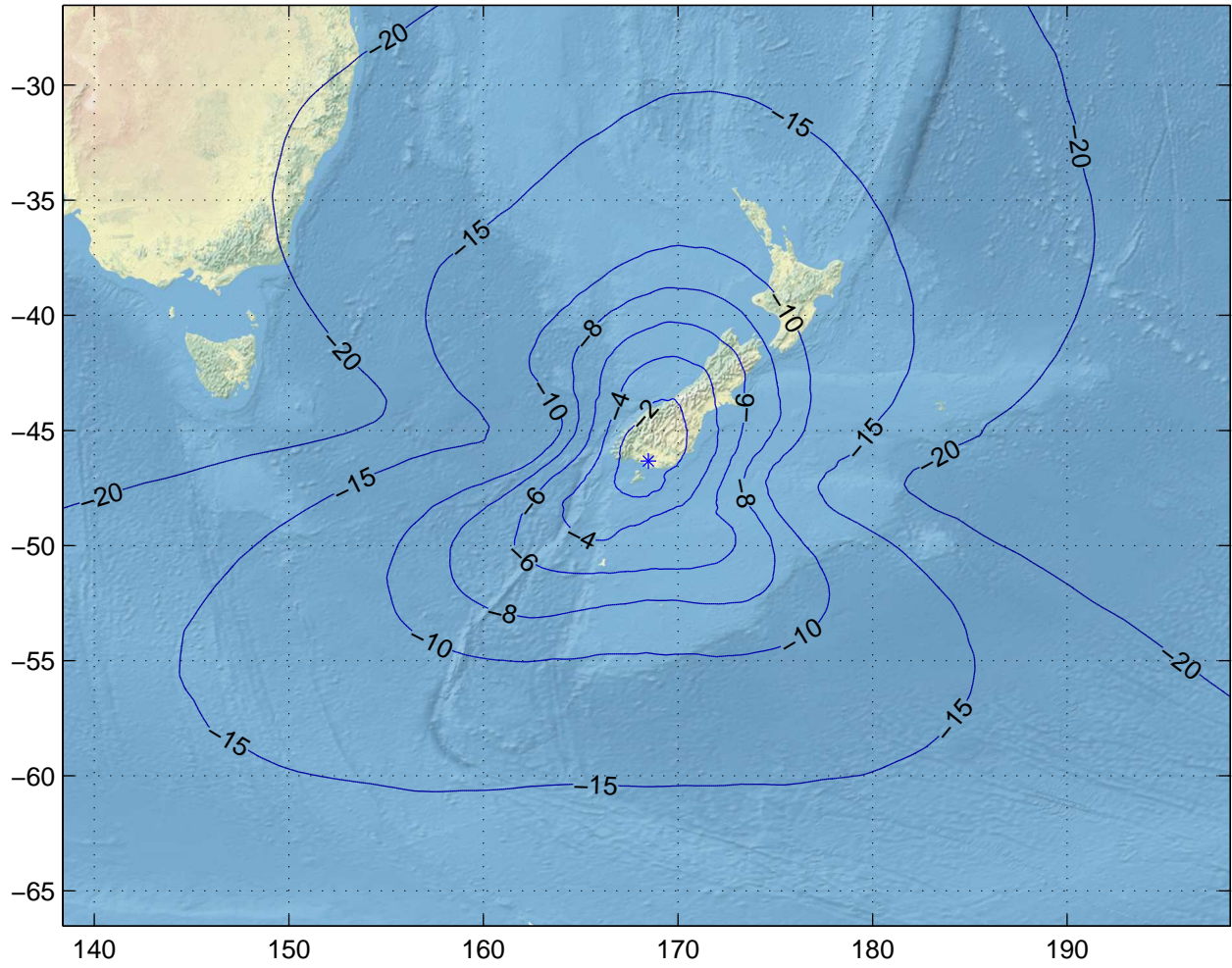
Gain Contours at 475km for IVC. Beam ID=SRX, Polarization=lhcp
