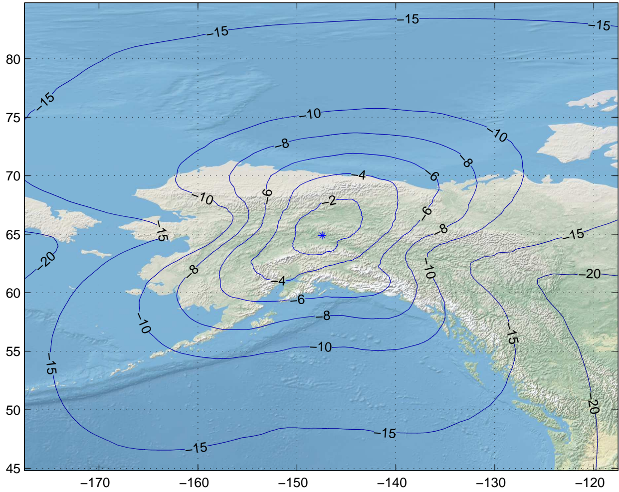
Gain Contours at 550km for FAI. Beam ID=SRX, Polarization=lhcp
